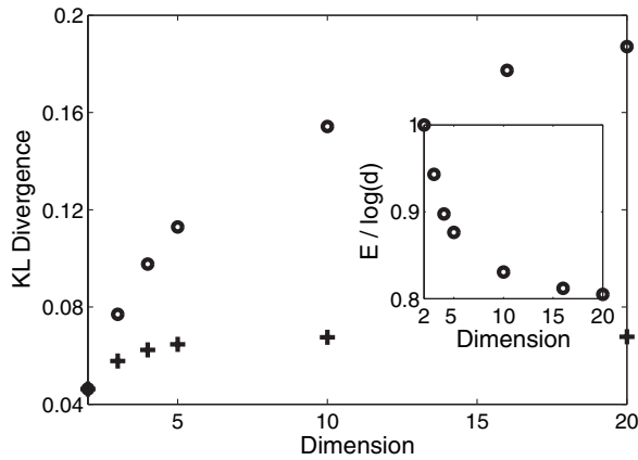
FIG. 1. KL divergence for Bell tests using two projective measurements under the mentioned assumptions. Circles correspond to the optimal state |\Psi_d\rangle , while crosses to the maximally entangled state |\Phi_d\rangle . In the inset, the entropy of entanglement for |\Psi_d\rangle is shown.
