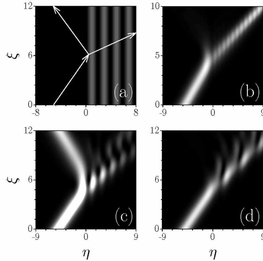
Fig. 1. (a) Schematic representation of the geometry of soliton refraction at the boundary between the lattice and uniform medium. Soliton propagation dynamics in illustrative cases, at \Omega = 8 (b), 3.5 (c), and 2 (d). In all cases \alpha_{\text{in}} = 1 , p = 1 , \chi = 1 .
