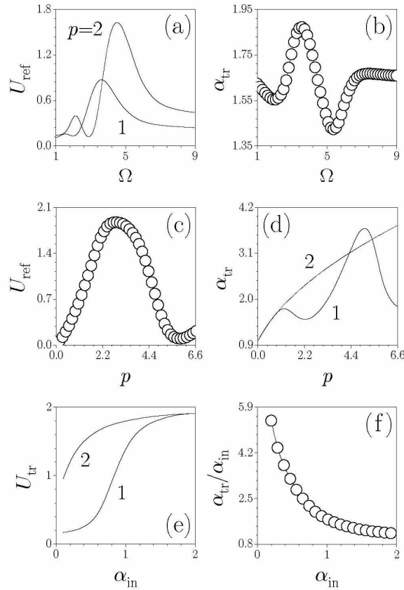
Fig. 2. (a) Reflected energy vs lattice frequency at \alpha_{in} = 1 . (b) Propagation angle of transmitted soliton vs lattice frequency at \alpha_{in} = 1 , p = 1 . (c) Reflected energy vs lattice depth at \alpha_{in} = 1 , \Omega = 4.2 . (d) Propagation angle of transmitted soliton vs lattice depth at \alpha_{in} = 1 , \Omega = 4.2 . Curve 1 – numerical results, curve 2 – analytical effective index approximation. (e) Energy of transmitted soliton vs incident angle at p = 1 , \Omega = 3 . Curve 1 – numerical results, curve 2 – analytical effective index approximation. (f) Ratio of propagation angles of transmitted and incident solitons versus incident angle at p = 1 , \Omega = 3 . In all cases \chi = 1 .
