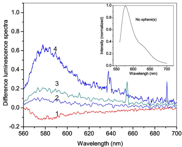
Fig. 2. (Color online) Difference spectra obtained with (1) an uncoated silica 2 \mu\text{m} sphere in the center of the 532 nm beam, (2) a single SPCM in the center of the 532 nm beam, and (3) and (4) a pair of SPCMs located symmetrically relative to the center of the 532 nm beam with two separation distances. The inset shows the normalized luminescence spectrum when no spheres are in the confocal volume.
