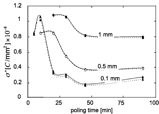
FIG. 4. Evolution of positive charge ( \sigma^+ ) on anodic surface for different sample thickness and poling time with solid and dashed line corresponding to \sigma_{hot}^+ and \sigma_{cold}^+ , respectively.
