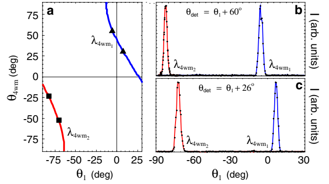
FIG. 3 (color online). Angular dependence of 4WM emission. (a) Calculated emission angles ( \theta_{4\text{wm}_1} , \theta_{4\text{wm}_2} ) as a function of excitation angle \theta_1 . The angle of \theta_2 is \theta_1 + 60^\circ . \lambda_1 = 707 nm, \lambda_2 = 800 nm, \lambda_{4\text{wm}_1} = 633 nm, and \lambda_{4\text{wm}_2} = 921 nm. (b), (c) Measured 4WM intensity as a function of excitation angle \theta_1 . The four resonance curves correspond to the angles marked by triangles in (a).
