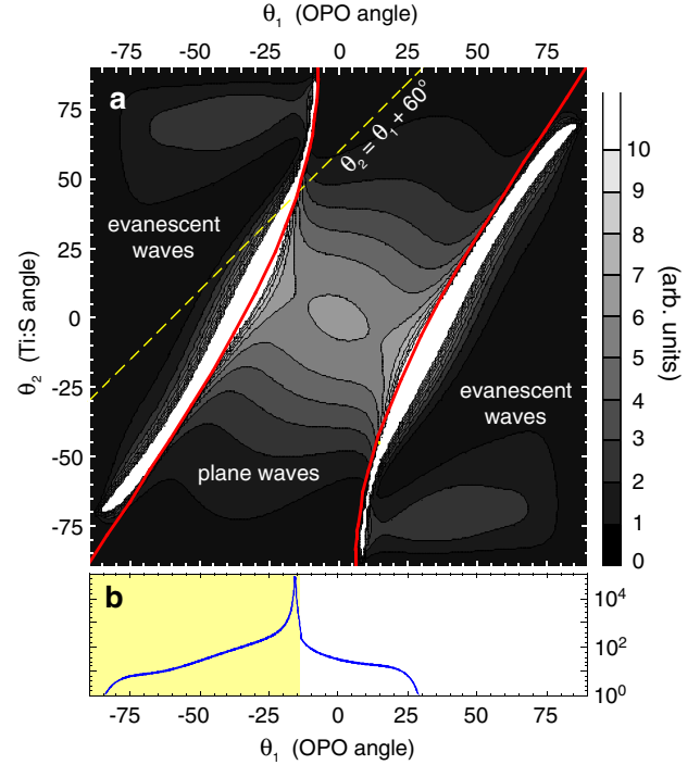
FIG. 2 (color online). (a) Efficiency of four-wave mixing ( |E_{4\text{wm}}|^2 ) at \lambda_{4\text{wm}_1} = 633 \text{ nm} as a function of excitation angles \theta_1 and \theta_2 . The solid line indicates the boundary between propagating and evanescent 4WM waves. (b) Line cut along the dashed line. The shaded area corresponds to the evanescent region. The intensity at the surface plasmon peak is more than 3 orders of magnitude larger than the intensity in the propagating region.
